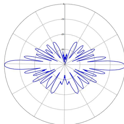
Vertical, 0° downtilt
